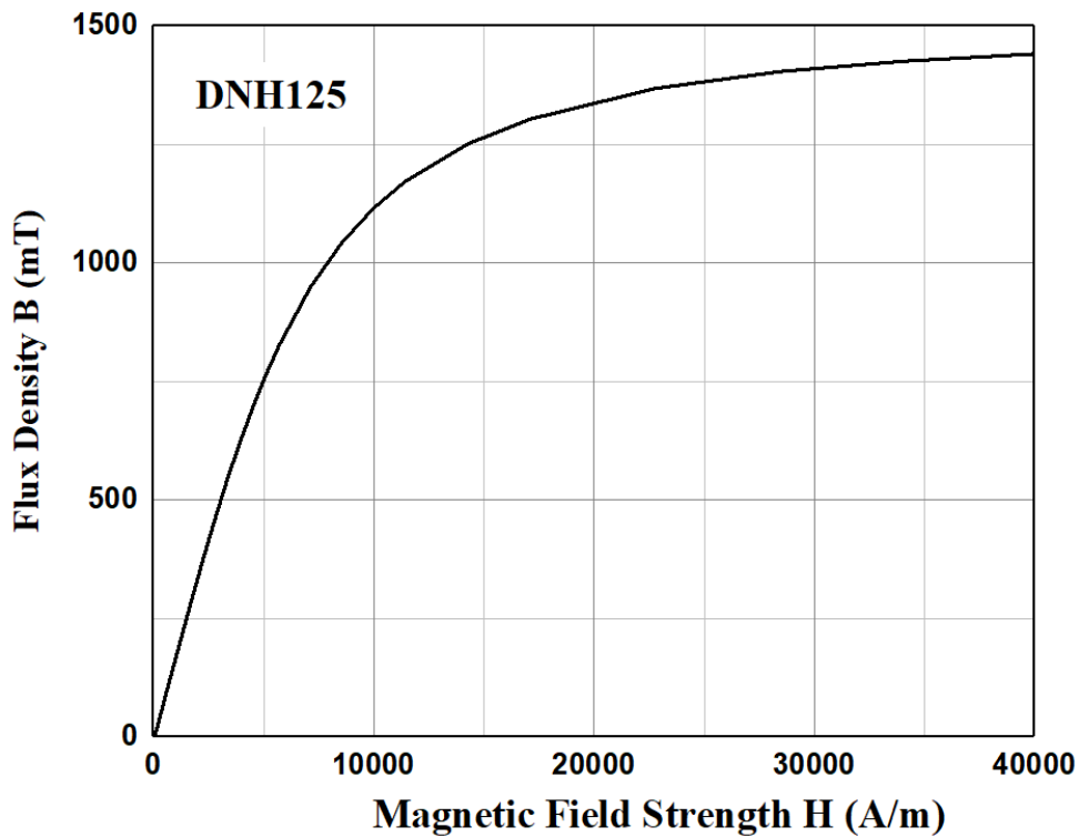
* 标准磁化曲线 Normal Magnetization Curve
